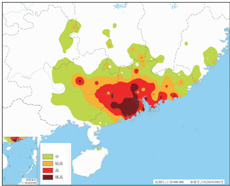
图 4 台风大风对输电线路致灾性评估模型对 2018 年 9 月 16—17 日“山竹”期间的致灾等级评估 Fig. 4 Disaster level assessment of Typhoon Mangkhut in 16—17 September 2018 based on the disaster assessment model for transmission lines under typhoon-generated strong wind
