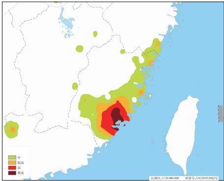
图 2 台风大风对输电线路致灾性评估模型对 2016 年 9 月 13—16 日“莫兰蒂”期间的致灾等级评估 Fig. 2 Disaster level assessment of Typhoon Meranti in 13—16 September 2016 based on the disaster assessment model for transmission lines under typhoon-generated strong wind
