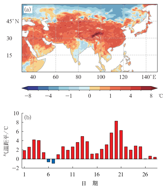
图 10 (a)2025/2026 年冬季亚洲地区气温距平空间分布及(b)2026 年 2 月我国内蒙古、甘肃、宁夏、新疆地区平均气温距平逐日演变 Fig. 10 (a) Spatial distribution of temperature anomaly in Asia in 2025/2026 winter, and (b) daily variation of average temperature anomaly in Inner Mongolia, Gansu, Ningxia, and Xinjiang in China in February 2026
