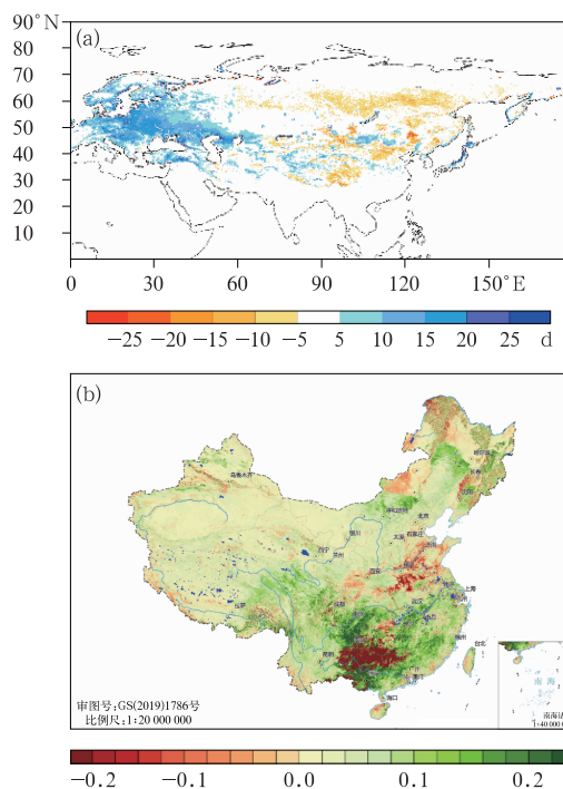
图 11 2026 年(a)1 月欧亚地区积雪日数距平及(b)2 月全国归一化植被指数距平分布 Fig. 11 Distribution of (a) anomaly of snow cover days over Eurasia in January, and (b) normalized vegetation index anomaly over China in February 2026
