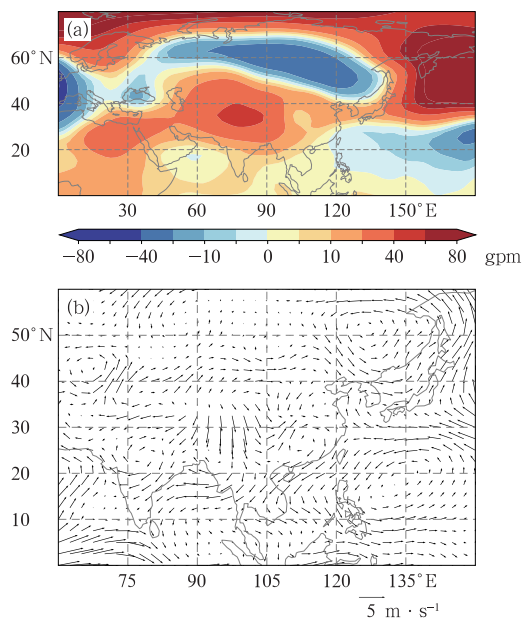
图 5 2025/2026 年冬季(a)500 hPa 位势高度距平场及(b)850 hPa 风场距平 Fig. 5 (a) The 500 hPa geopotential height anomaly and (b) 850 hPa wind anomaly in the 2025/2026 winter
